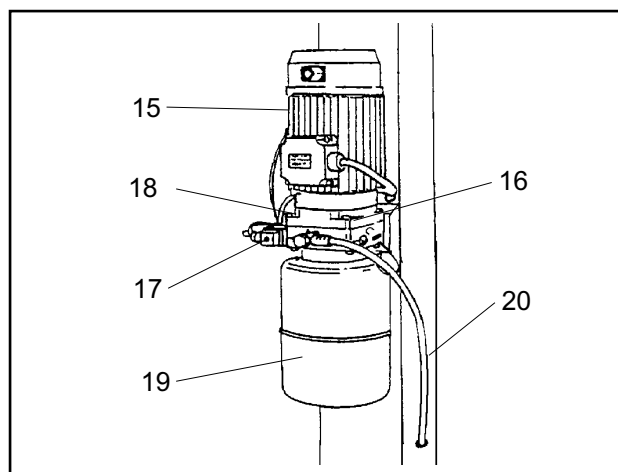
Fig.8 Centralina idraulica Fig.8 Hydraulic power unit
