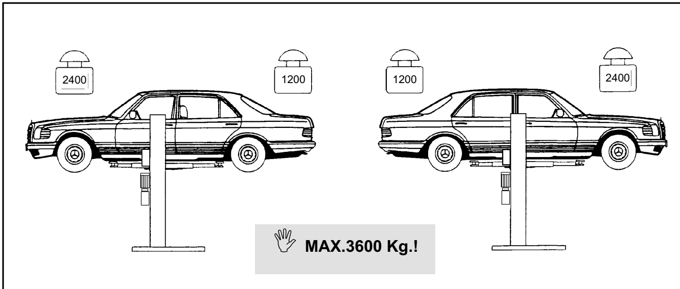
Fig.14 Weight distribution
