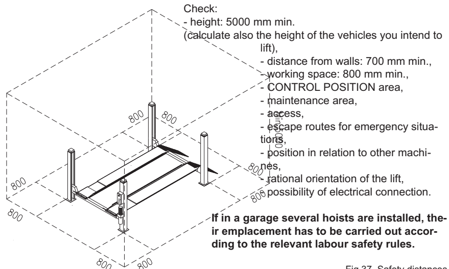
Fig.37 Safety distances
