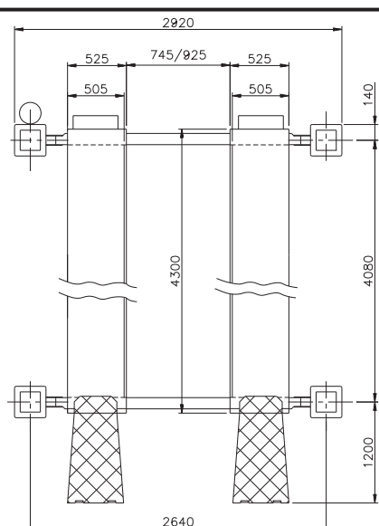
Fig.11a - Overall dimensions and clearances with platforms without recess for wheel alignment
